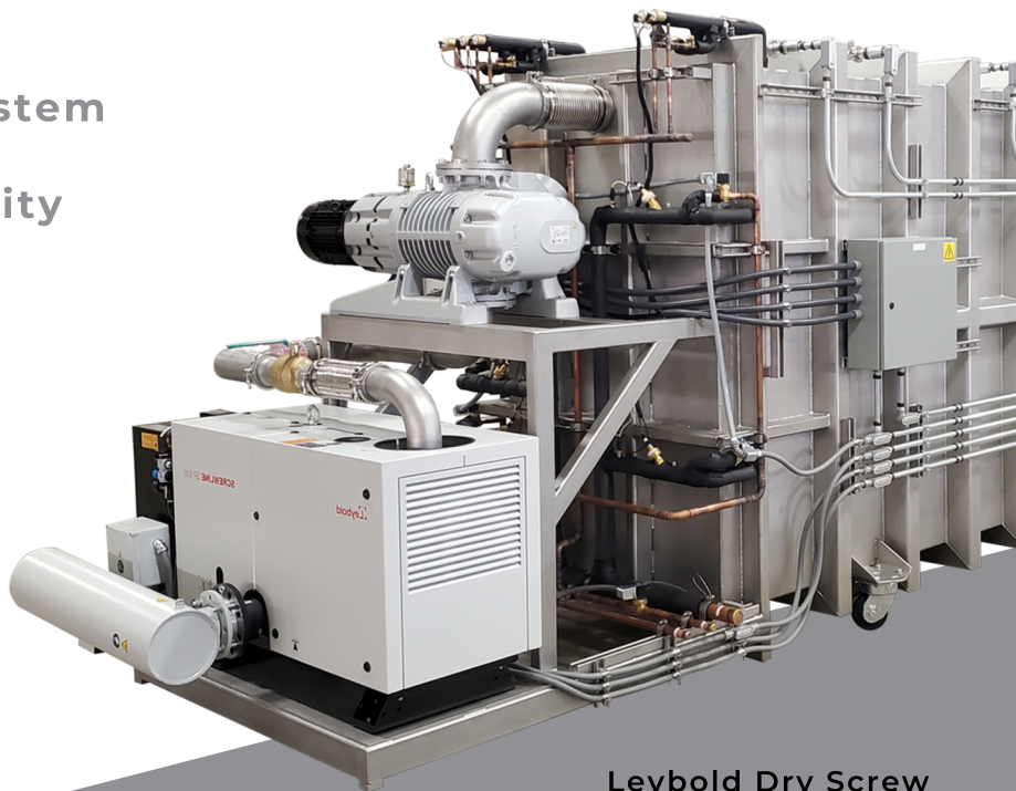
Leybold Dry Screw Pump and Booster
