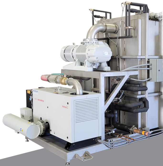
Leybold Dry Screw Pump and Booster
